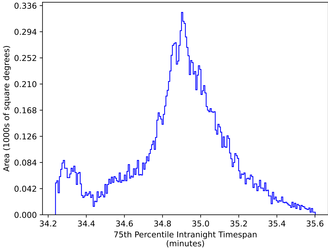
too_elab_r16_d2_griz_v3.4_10yrs WFD: 75th Percentile Intranight Timespan
