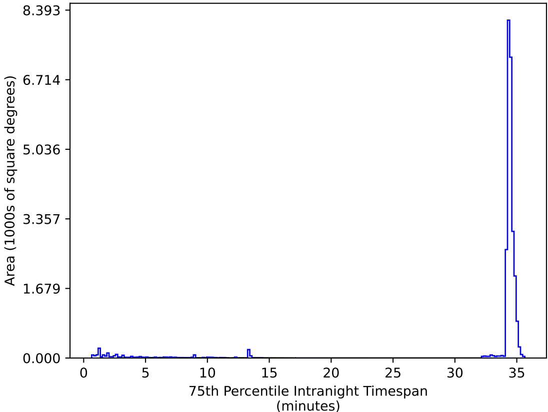
too_elab_r16_d2_griz_v3.4_10yrs All sky zy bands: 75th Percentile Intranight Timespan
