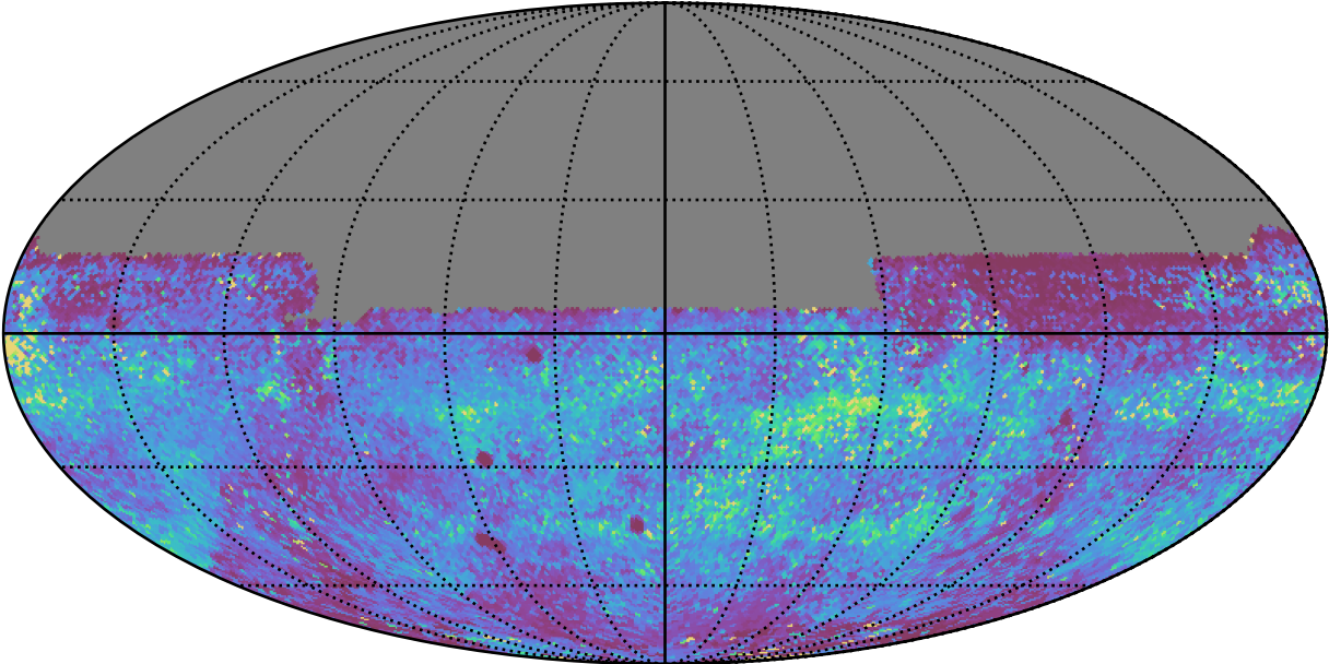
too_elab_r16_d2_griz_v3.4_10yrs All sky y band: 75th Percentile Intranight Timespan
