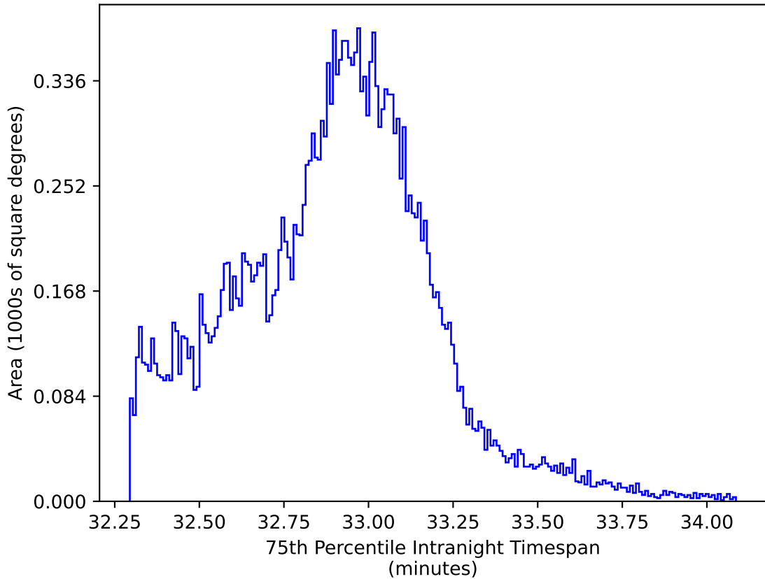
too_elab_r16_d2_griz_v3.4_10yrs All sky y band: 75th Percentile Intranight Timespan
