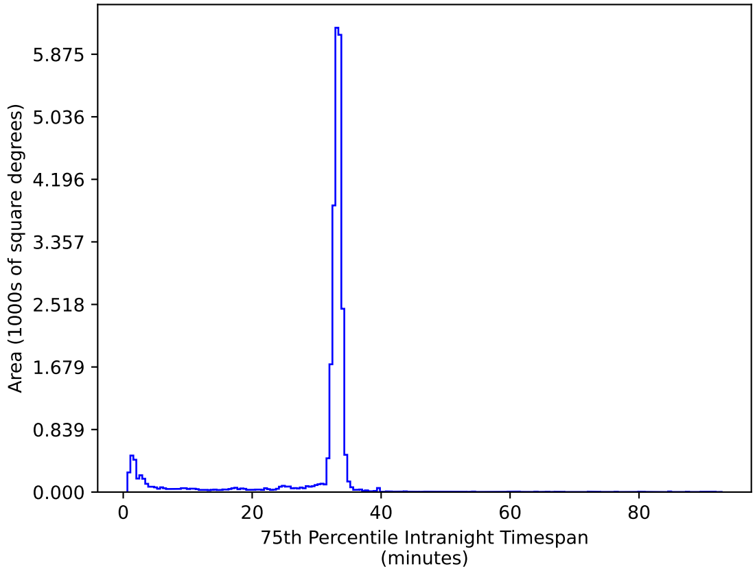
too_elab_r16_d2_griz_v3.4_10yrs All sky ug bands: 75th Percentile Intranight Timespan
