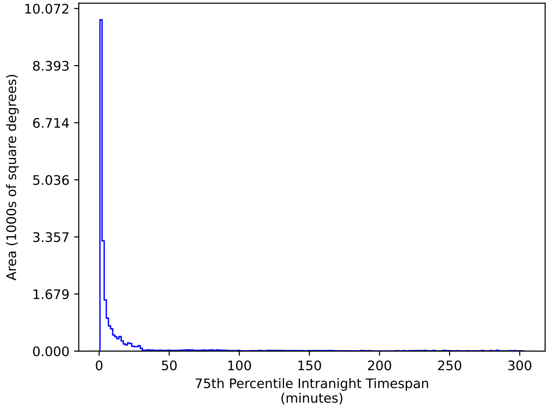
too_elab_r16_d2_griz_v3.4_10yrs All sky u band: 75th Percentile Intranight Timespan
