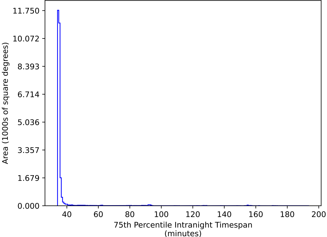
too_elab_r16_d2_griz_v3.4_10yrs All sky ri bands: 75th Percentile Intranight Timespan
