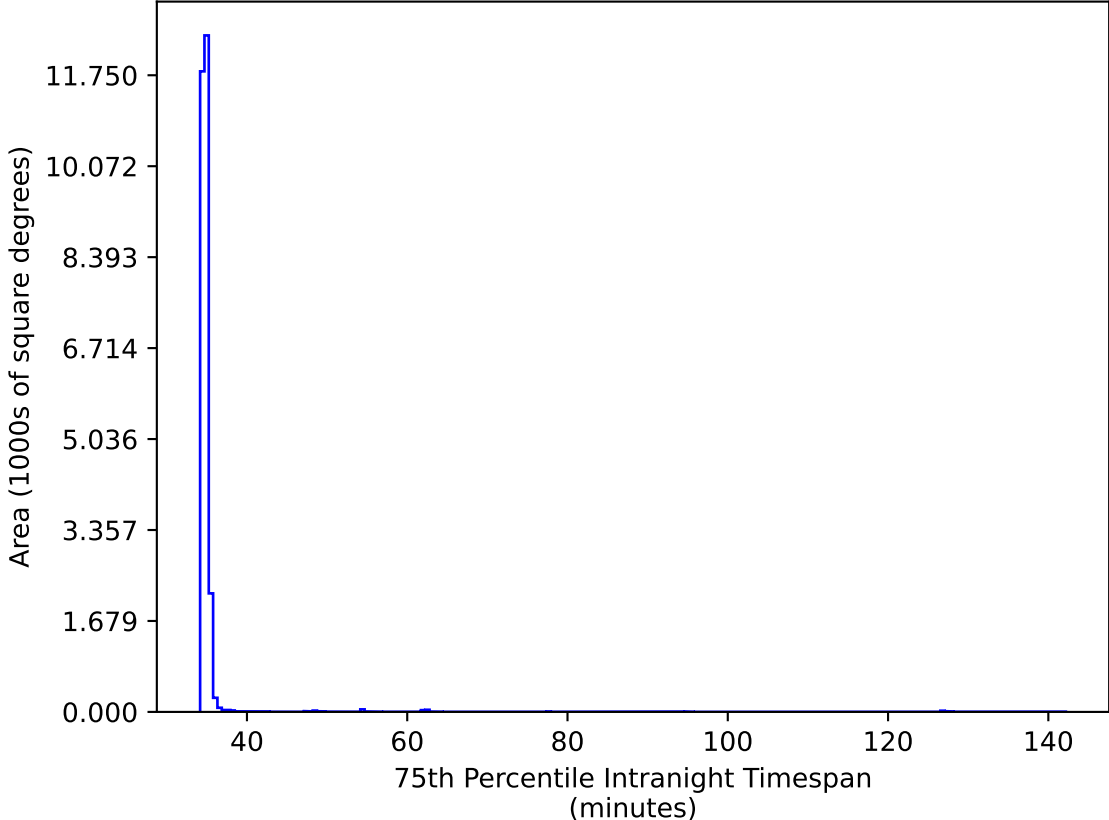
too_elab_r16_d2_griz_v3.4_10yrs All sky iz bands: 75th Percentile Intranight Timespan
