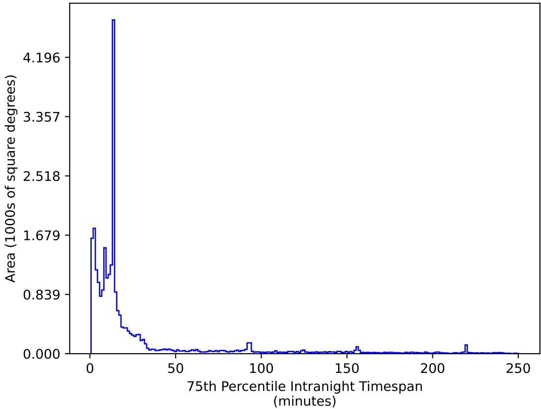
too_elab_r16_d2_griz_v3.4_10yrs All sky i band: 75th Percentile Intranight Timespan
