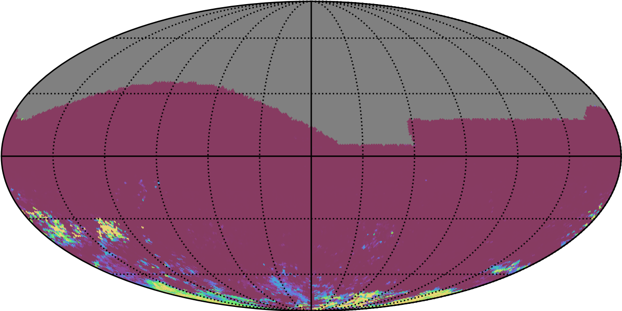
too_elab_r16_d2_griz_v3.4_10yrs All sky gr bands: 75th Percentile Intranight Timespan
