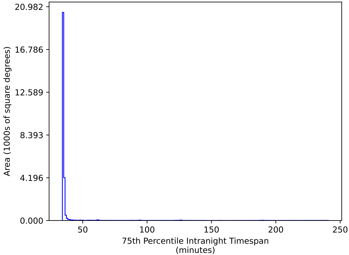
too_elab_r16_d2_griz_v3.4_10yrs All sky gr bands: 75th Percentile Intranight Timespan
