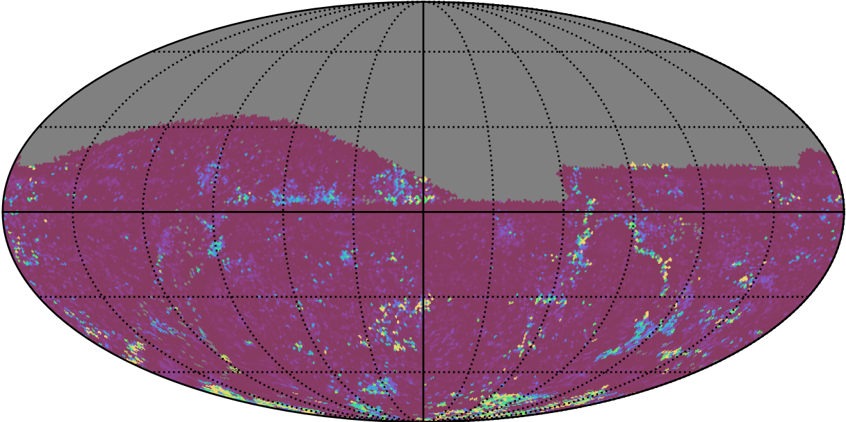
too_elab_r16_d2_griz_v3.4_10yrs All sky g band: 75th Percentile Intranight Timespan
