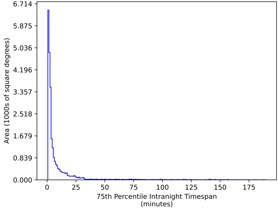
too_elab_r16_d2_griz_v3.4_10yrs All sky g band: 75th Percentile Intranight Timespan
