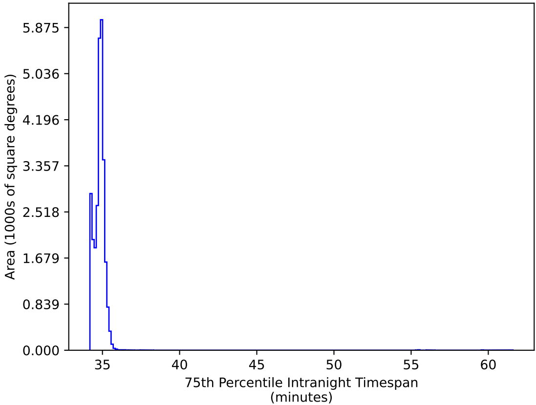
too_elab_r16_d2_griz_v3.4_10yrs All sky all bands: 75th Percentile Intranight Timespan
