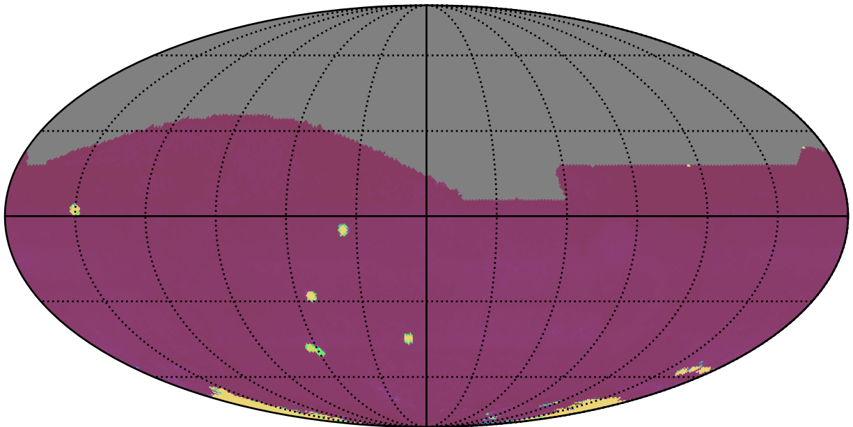
too_elab_r16_d2_griz_v3.4_10yrs All sky: 75th Percentile Intranight Timespan
