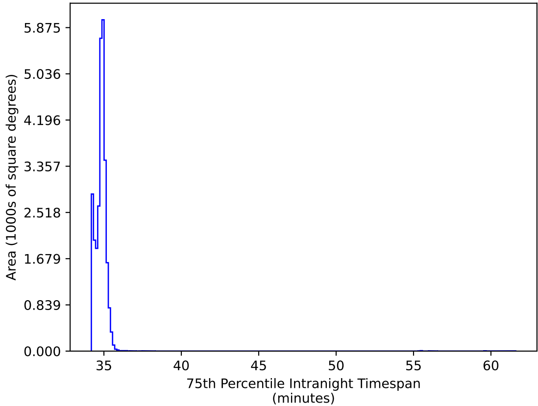
too_elab_r16_d2_griz_v3.4_10yrs All sky: 75th Percentile Intranight Timespan
