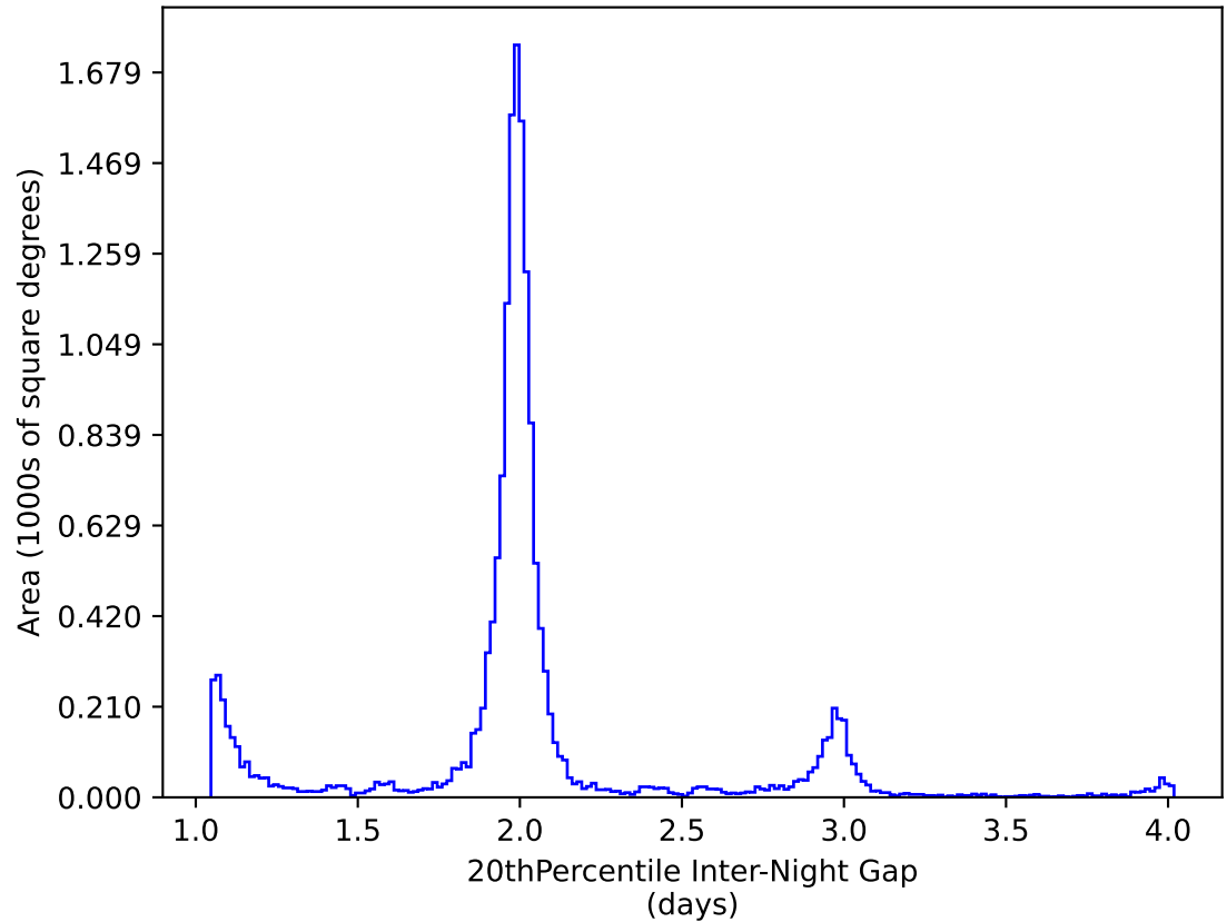
too_elab_r16_d2_griz_v3.4_10yrs WFD y band: 20thPercentile Inter-Night Gap
