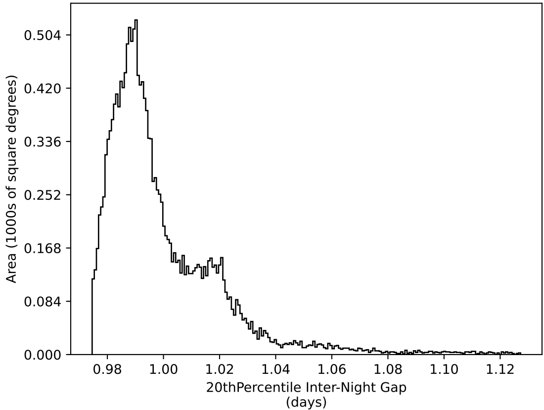
too_elab_r16_d2_griz_v3.4_10yrs WFD all bands: 20thPercentile Inter-Night Gap
