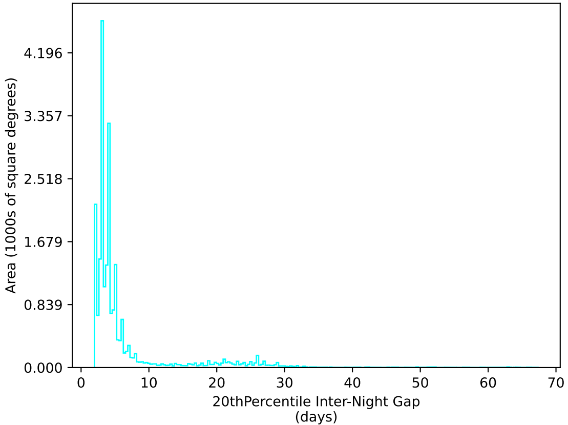
too_elab_r16_d2_griz_v3.4_10yrs All sky u band: 20thPercentile Inter-Night Gap
