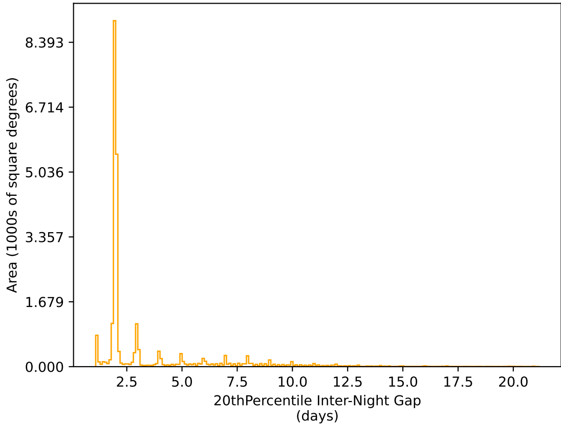
too_elab_r16_d2_griz_v3.4_10yrs All sky r band: 20thPercentile Inter-Night Gap
