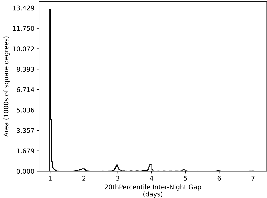
too_elab_r16_d2_griz_v3.4_10yrs All sky all bands: 20thPercentile Inter-Night Gap
