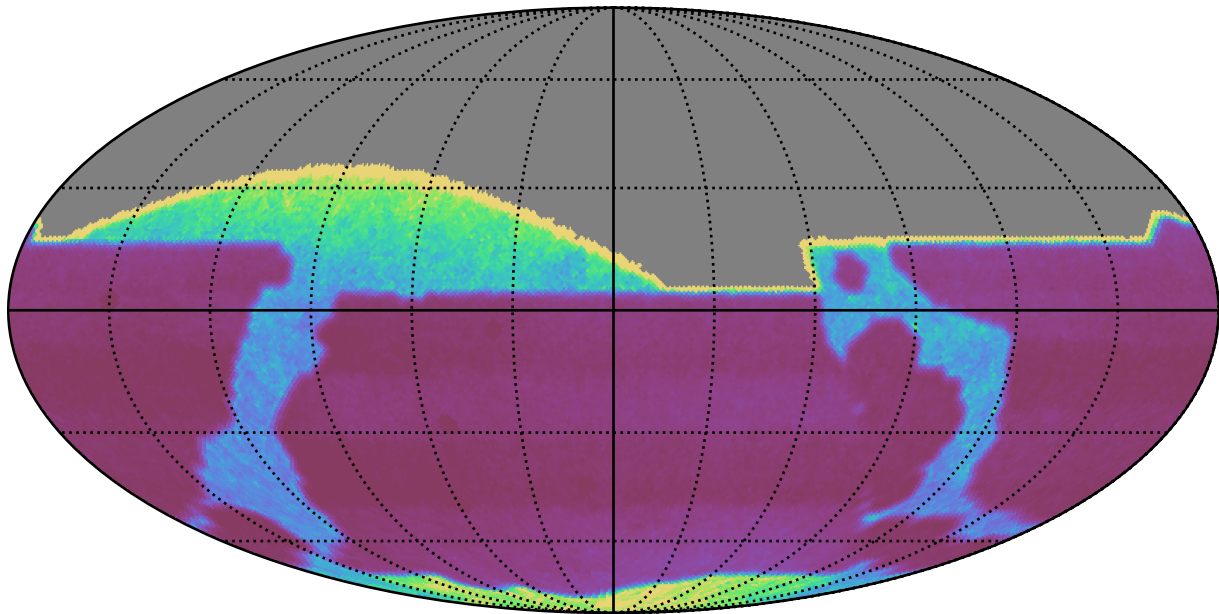
too_elab_r16_d2_griz_v3.4_10yrs : properMotion
