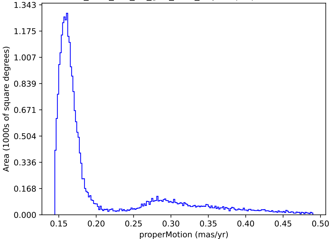
too_elab_r16_d2_griz_v3.4_10yrs : properMotion
