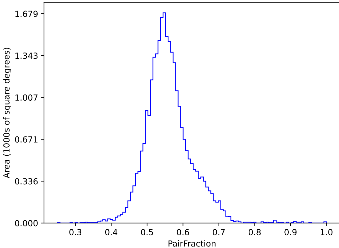
too_elab_r16_d2_griz_v3.4_10yrs (g or r or i): PairFraction
