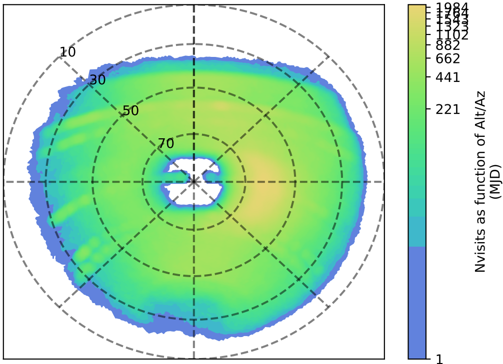
too_elab_r16_d2_griz_v3.4_10yrs y: Nvisits as function of Alt/Az
