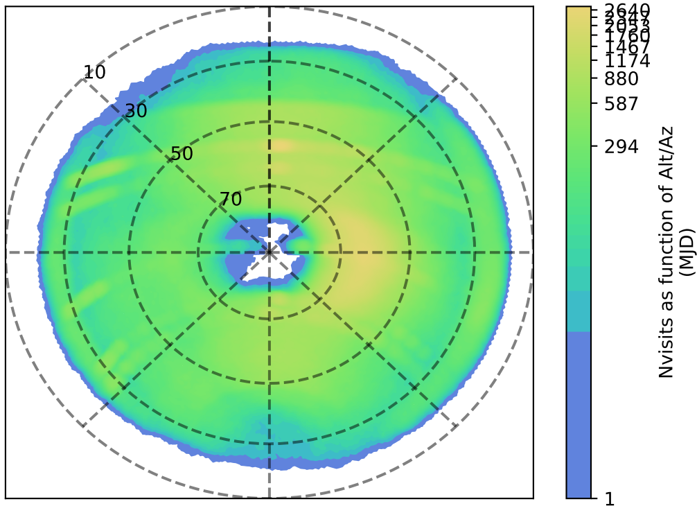
too_elab_r16_d2_griz_v3.4_10yrs i: Nvisits as function of Alt/Az
