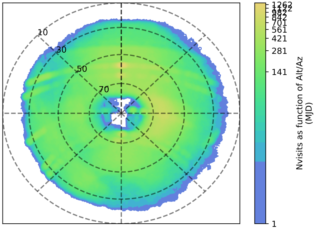
too_elab_r16_d2_griz_v3.4_10yrs g: Nvisits as function of Alt/Az
