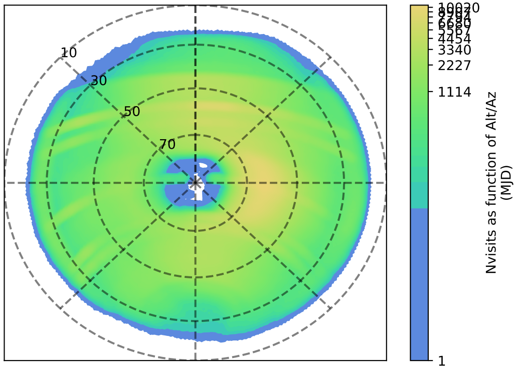
too_elab_r16_d2_griz_v3.4_10yrs : Nvisits as function of Alt/Az
