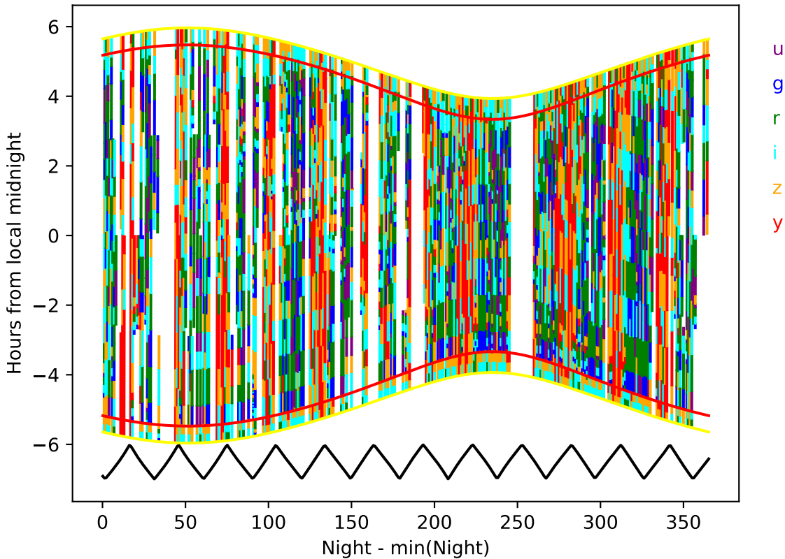
too_elab_r16_d2_griz_v3.4_10yrs year 5-6: Hourglass
