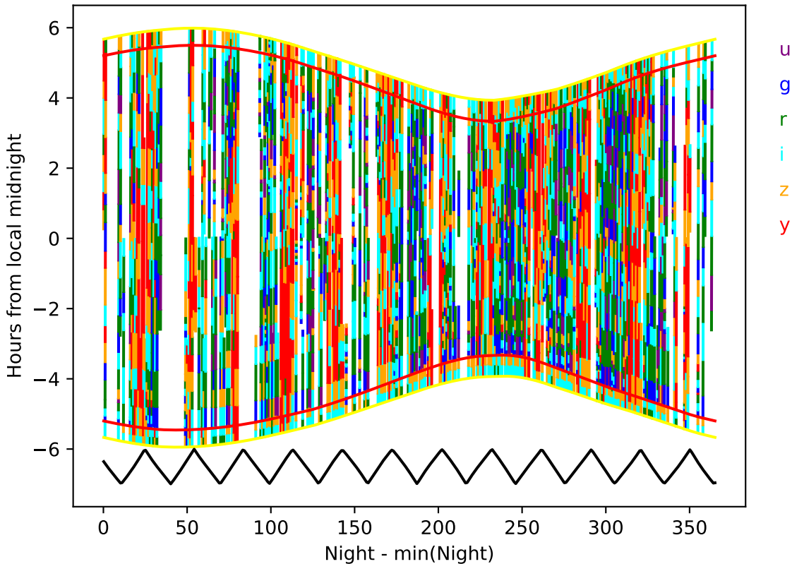
too_elab_r16_d2_griz_v3.4_10yrs year 4-5: Hourglass
