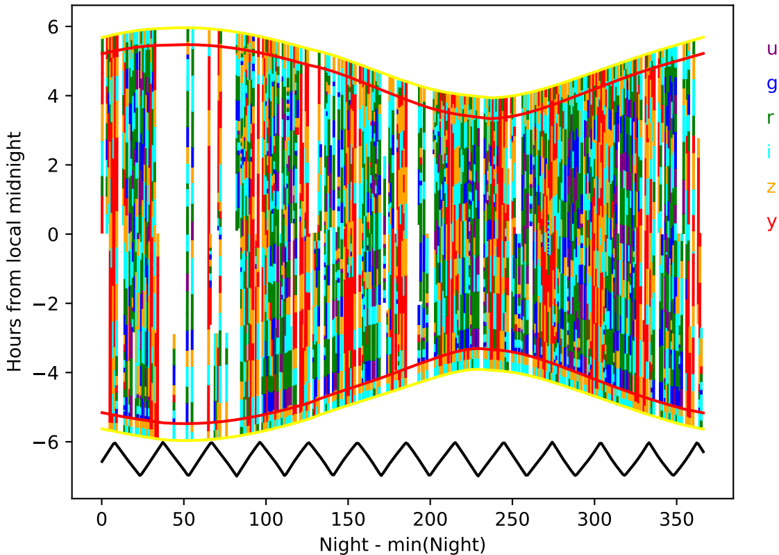
too_elab_r16_d2_griz_v3.4_10yrs year 3-4: Hourglass
