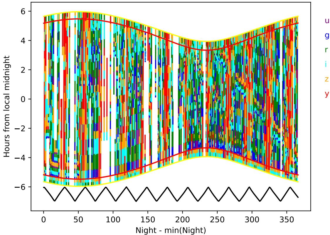
too_elab_r16_d2_griz_v3.4_10yrs year 1-2: Hourglass
