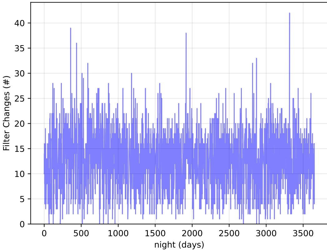
too_elab_r16_d2_griz_v3.4_10yrs : Filter Changes
