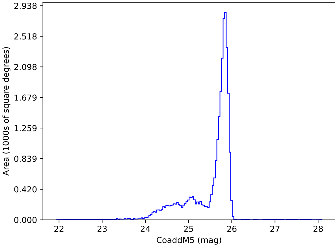
too_elab_r16_d2_griz_v3.4_10yrs z: CoaddM5
