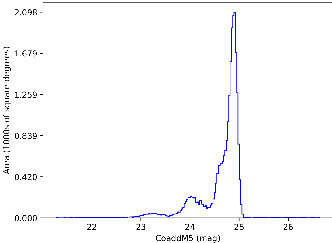
too_elab_r16_d2_griz_v3.4_10yrs y: CoaddM5
