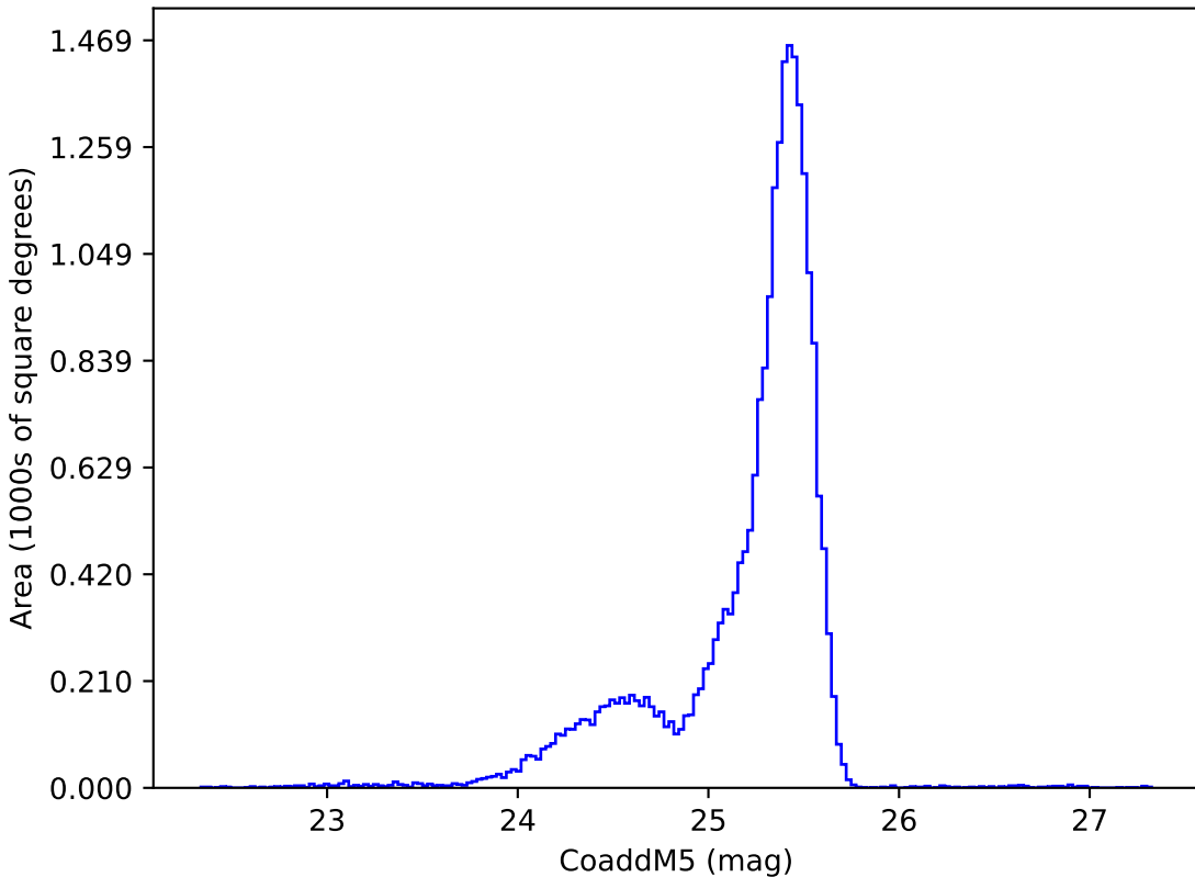
too_elab_r16_d2_griz_v3.4_10yrs u: CoaddM5
