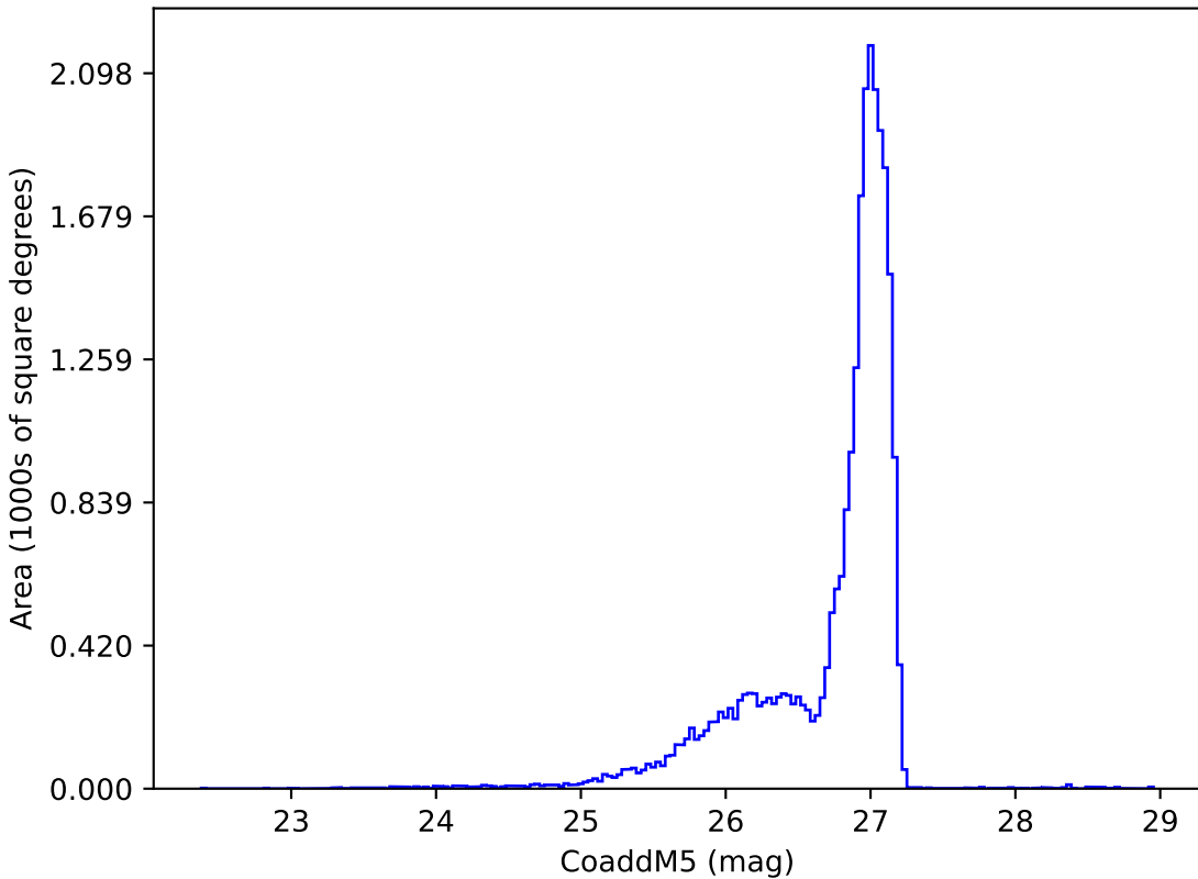
too_elab_r16_d2_griz_v3.4_10yrs r: CoaddM5
