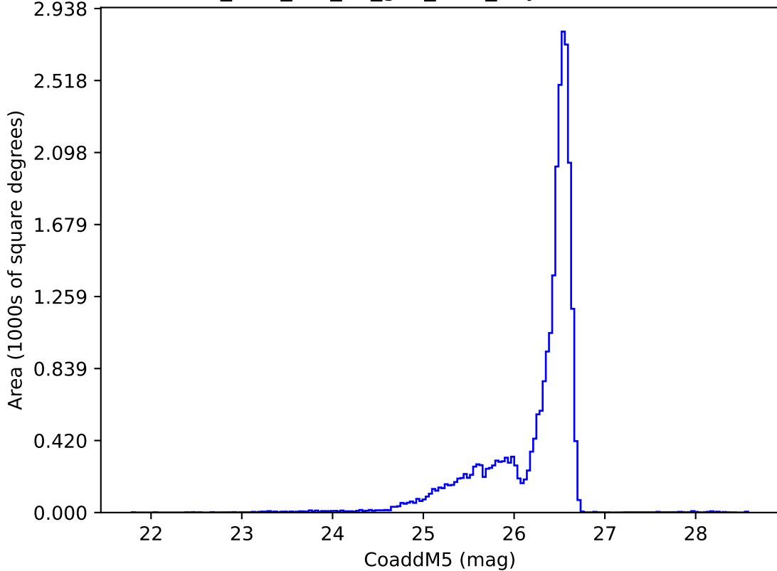
too_elab_r16_d2_griz_v3.4_10yrs i: CoaddM5
