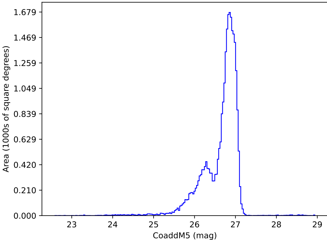
too_elab_r16_d2_griz_v3.4_10yrs g: CoaddM5
