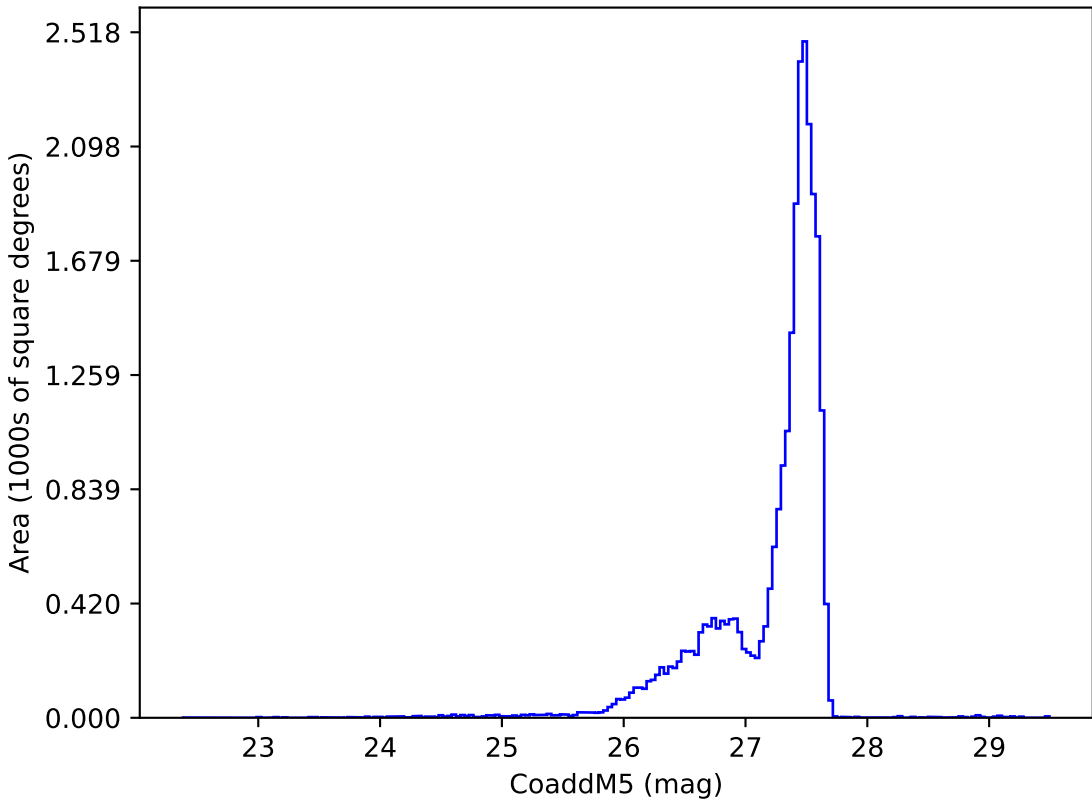
too_elab_r16_d2_griz_v3.4_10yrs : CoaddM5
