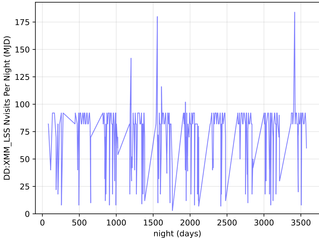
too_elab_r16_d2_griz_v3.4_10yrs all bands: DD:XMM_LSS Nvisits Per Night
