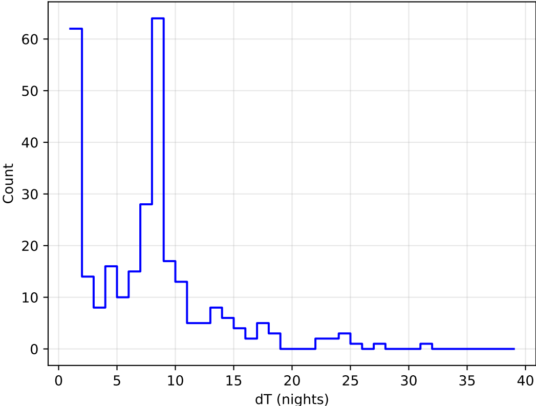
too_elab_r16_d2_griz_v3.4_10yrs all bands: DD:XMM_LSS Delta Nights Histogram
