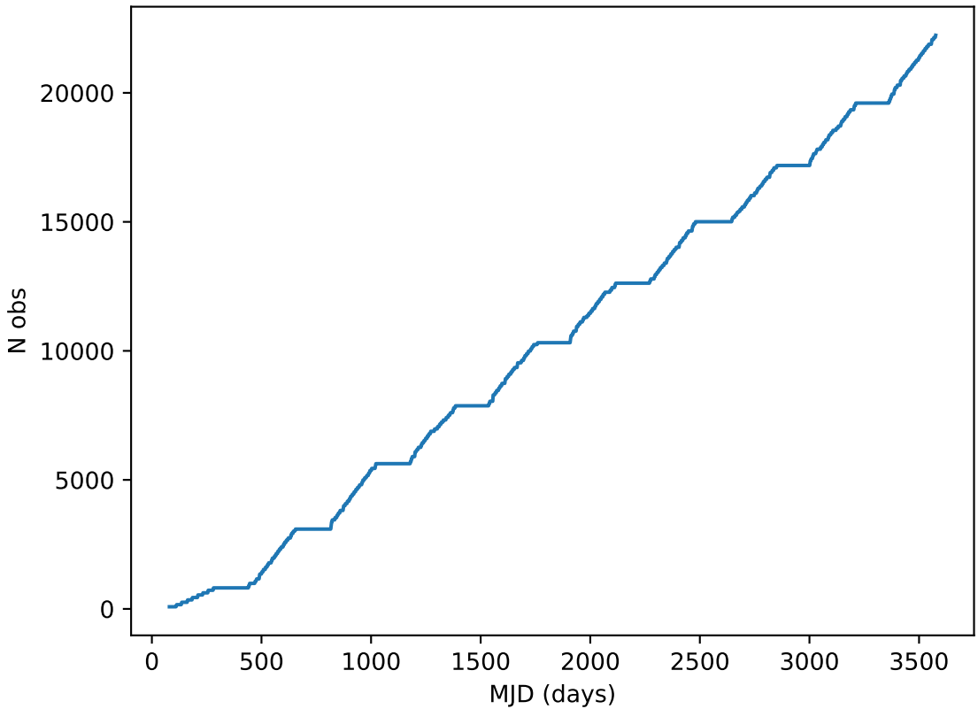
too_elab_r16_d2_griz_v3.4_10yrs all bands: DD:XMM_LSS Cumulative NVisits
