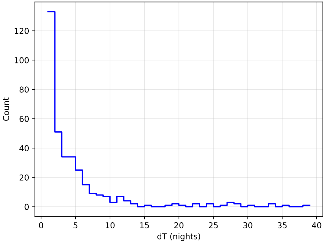
too_elab_r16_d2_griz_v3.4_10yrs all bands: DD:WFD Delta Nights Histogram
