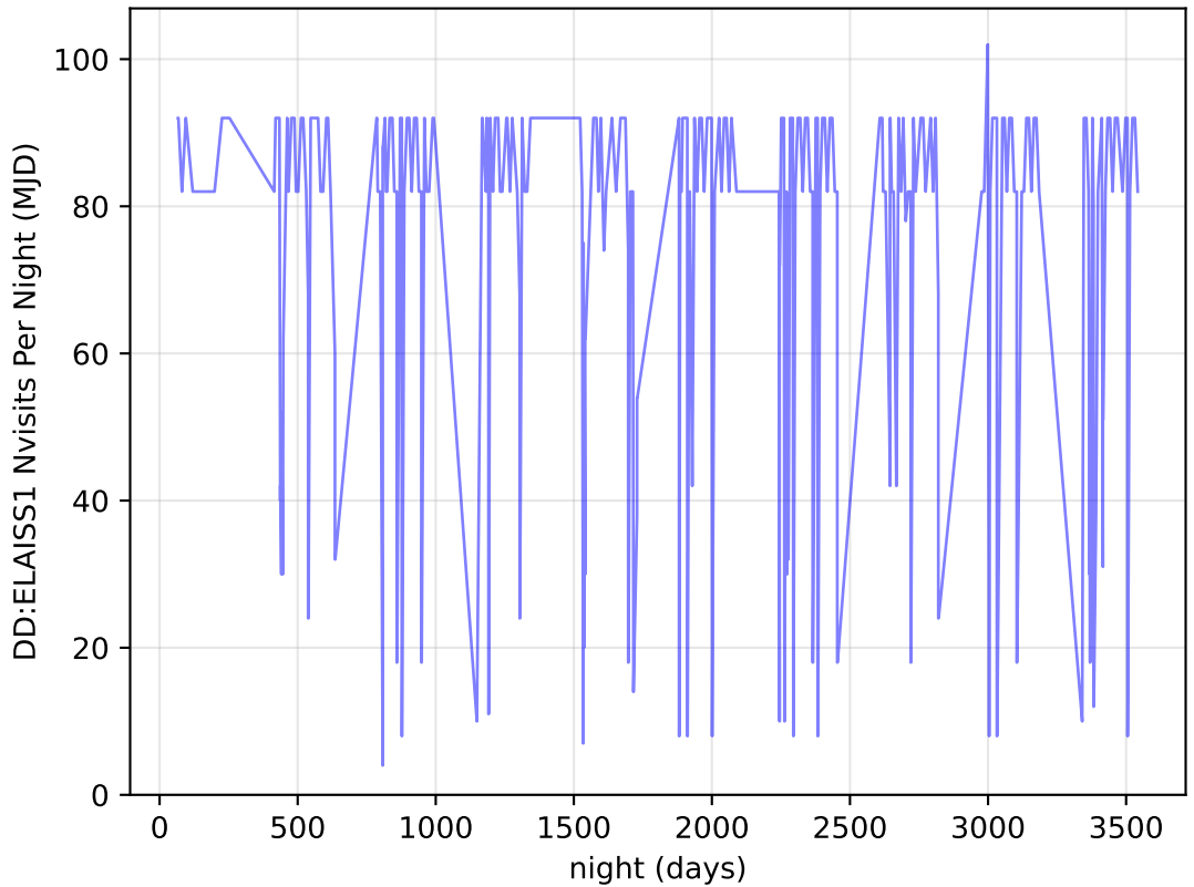
too_elab_r16_d2_griz_v3.4_10yrs all bands: DD:ELAISS1 Nvisits Per Night
