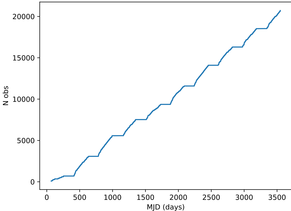
too_elab_r16_d2_griz_v3.4_10yrs all bands: DD:ELAISS1 Cumulative NVisits
