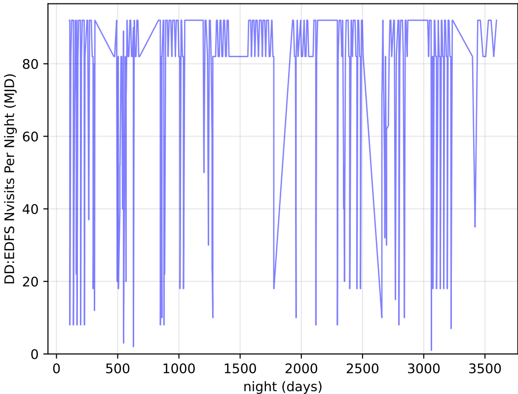
too_elab_r16_d2_griz_v3.4_10yrs all bands: DD:EDFS Nvisits Per Night
