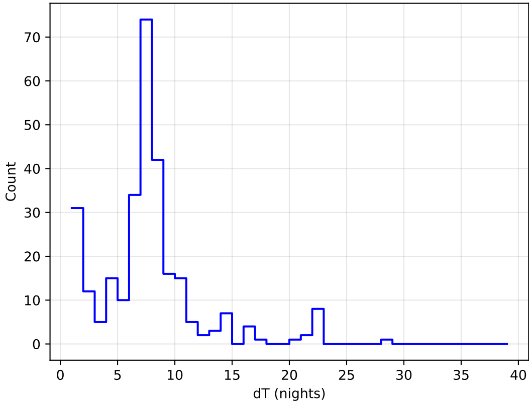
too_elab_r16_d2_griz_v3.4_10yrs all bands: DD:EDFS Delta Nights Histogram
