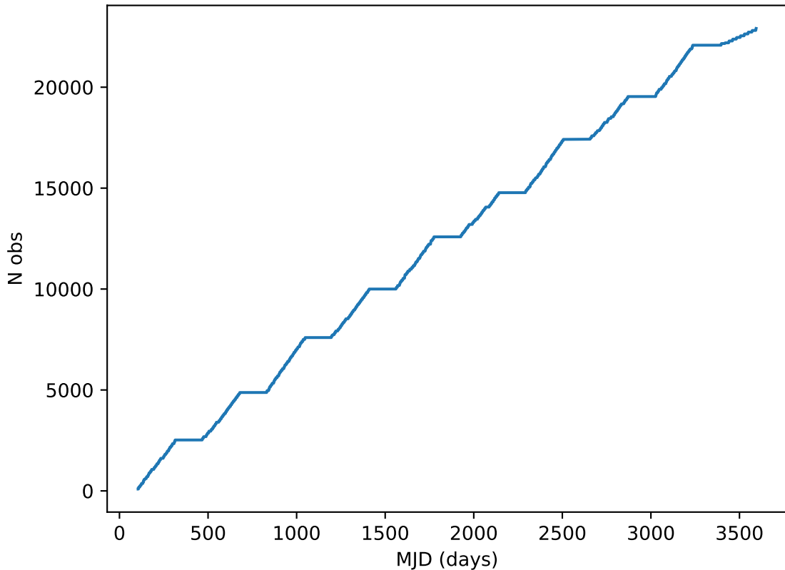
too_elab_r16_d2_griz_v3.4_10yrs all bands: DD:EDFS Cumulative NVisits
