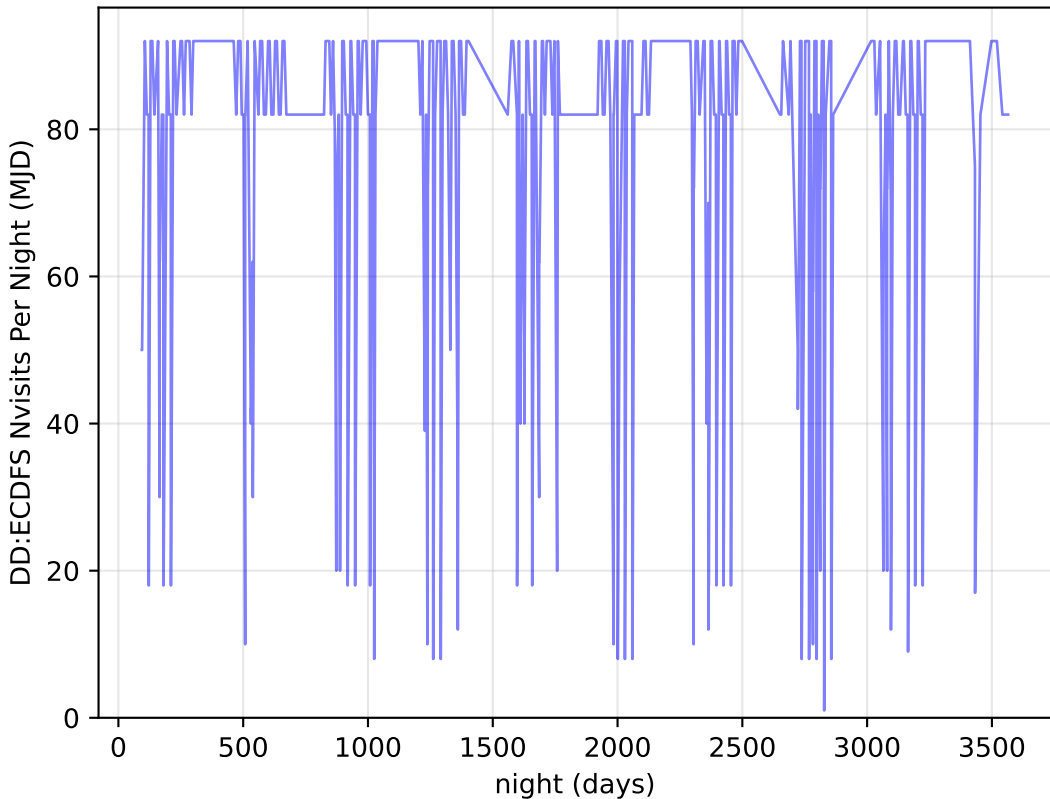
too_elab_r16_d2_griz_v3.4_10yrs all bands: DD:ECDFS Nvisits Per Night
